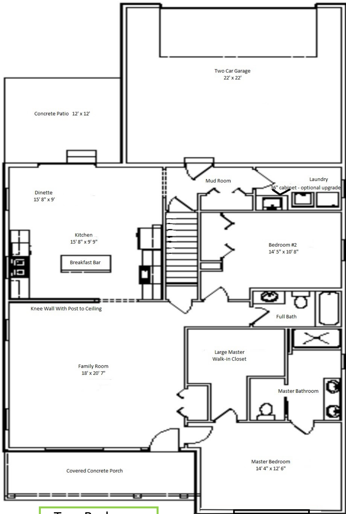
Two Bedroom 1573 Sq. Ft.
